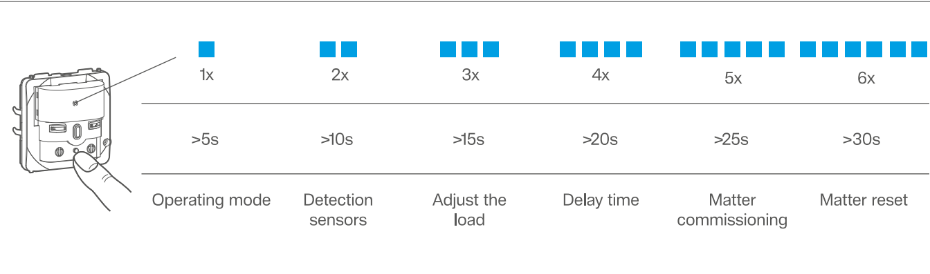
Fig. 12: Selection of special functions and status LED
